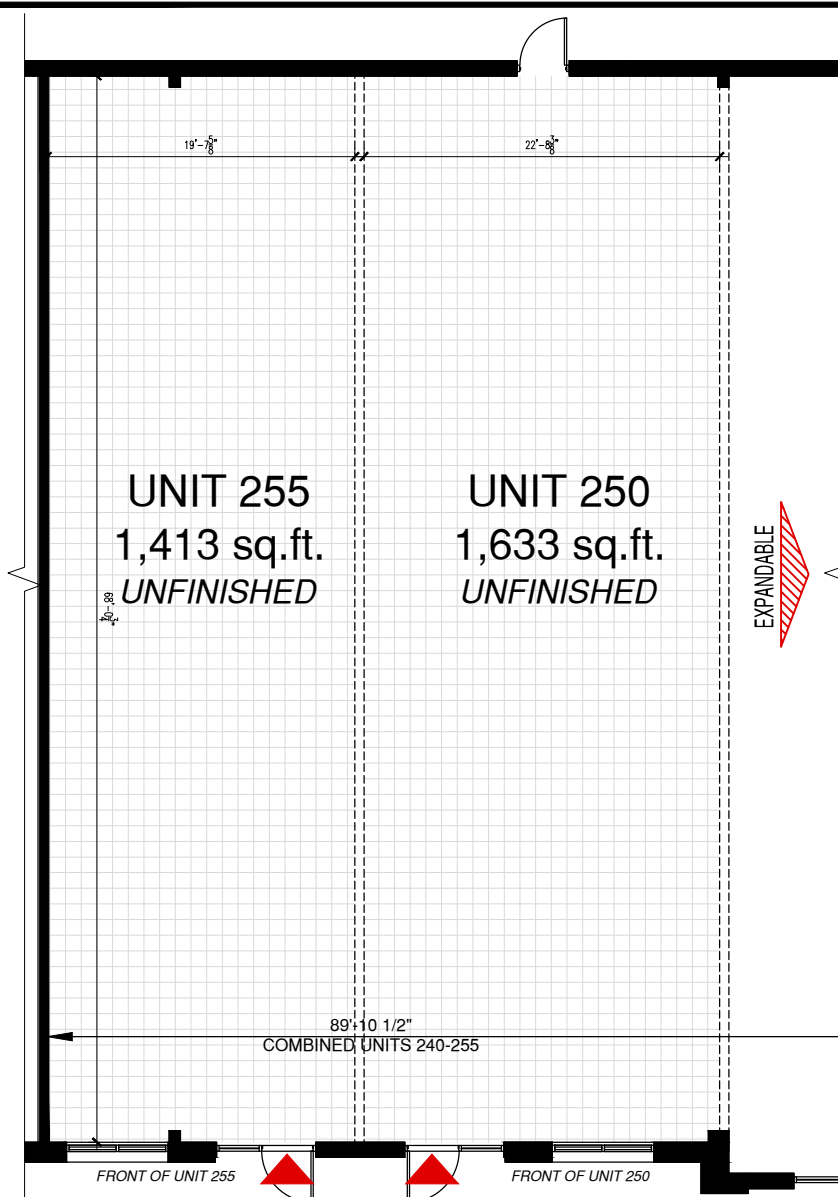
FLOOR PLAN - UNITS 250 & 255 SCALE: 3/16" = 1'-0"
