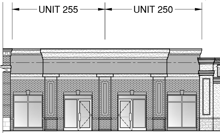
ELEVATION - UNITS 250 & 255 SCALE: 3/16" = 1'-0"
